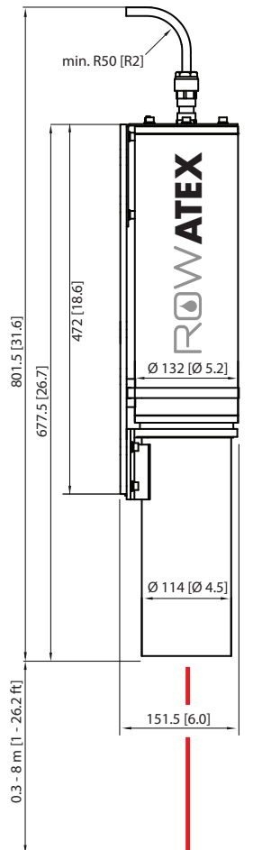
Dimensions unless otherwise stated: mm [inches]
