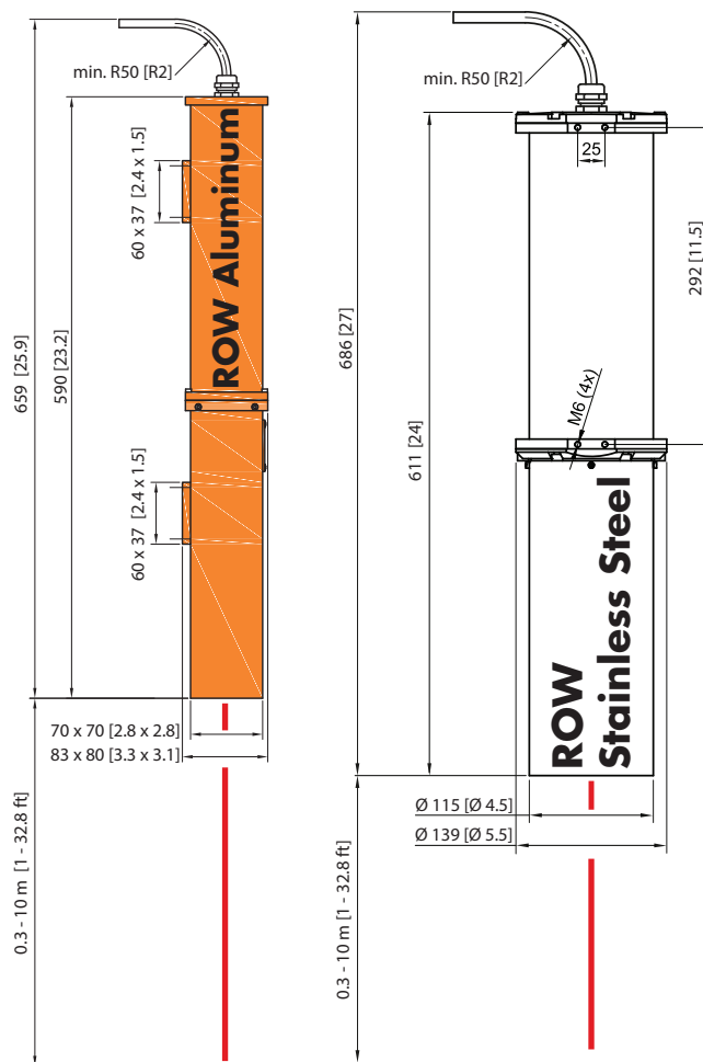
Dimensions unless otherwise stated: mm [inches]
